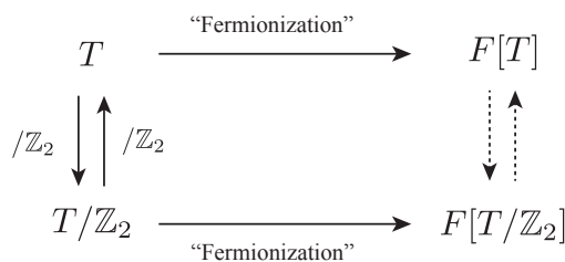
Figure 4: The interplay between fermionization and gauging \mathbb{Z}_2 symmetry. The downward arrow on the left denotes gauging the \mathbb{Z}_2 (n - 1) -form symmetry in T , while the upward arrow on the left denotes gauging the dual \mathbb{Z}_2 (n - 1) -form symmetry in F[T] . On the right, the downward arrow and upward arrow denotes stacking with the invertible phase in Section 4 or its complex conjugate, together with a change in the symmetry fractionalization as discussed in (96).
