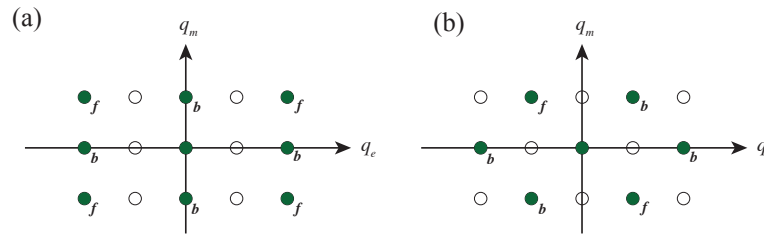
Figure 2: The genuine line operators of the SO(3)_+ and the SO(3)_- theories (both with \theta = 0 ) are marked as the green dots in the integer lattice (q_e, q_m) . The letters “b” and “f” indicates the bosonic and fermionic statistics of the corresponding line.
