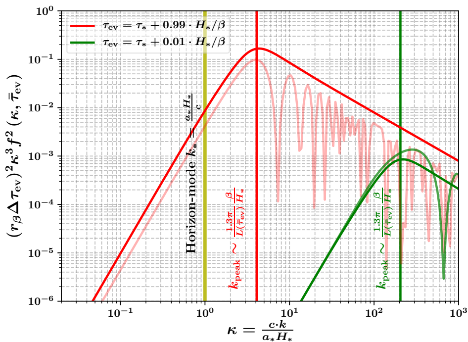
Figure 3: The dimensionless power spectrum of GWs sourced by a FPT (light red and light green) and the approximation of the time integral in Eq. (64) (bold lines) close to the start and the end of the FPT. The yellow curve shows the horizon mode. The notation is the same as in Fig. 2.
