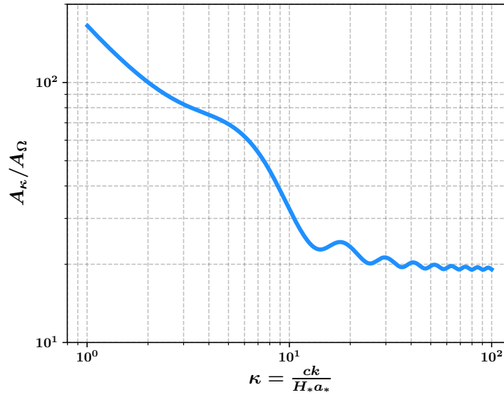
Figure 14: Ratio between the amplitudes in Eqs. (C.9) and (C.10) evaluated at t_{eq} for a benchmark strong PT with \alpha \rightarrow \infty , r_\beta = 1 and t_* = 10^{10} s. Note that the ratio is always bigger than 20, meaning that the solution sourced by the decaying GW source after t_f can be safely neglected in Eq. (82).
