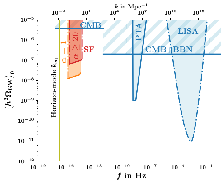
Figure 13: The GW abundance today as a function of today frequency. Shown are the projected bound by LISA [2] (dashed-dot blue), the bound set by PTAs [64–67] (solid blue) and the indirect bounds from CMB and BBN [68–70] (hatched areas). As the result of our calculation, the red colored regions are excluded by structure formation. However, many assumptions went into our calculation so the bound should be taken with care.
