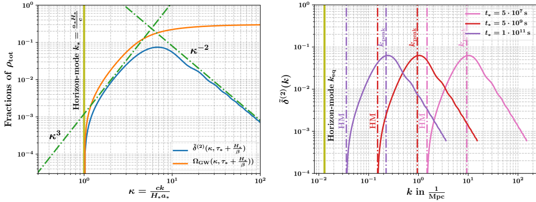
Figure 6: Left: In blue the numerical solution of Eq. (84) at the end of the phase transition and with initial conditions \tilde{\delta}^{(2)}(\kappa, t) = \tilde{\delta}^{(2)\prime}(\kappa, t) = 0 and for \alpha \rightarrow \infty and \beta/H_* = 1 . We also show the source term in orange at the end of the phase transition \tau_{\text{ev}} = \tau_* + H_*/\beta . Right: Induced density perturbation by GWs from FPT. For demonstration purposes we chose \alpha \rightarrow \infty, \beta = H_* . Shown are solutions for different scales a_*H_* in comparison with the horizon at matter-radiation equality.
