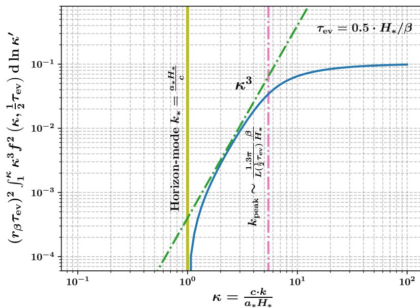
Figure 5: The integrated dimensionless power spectrum of GWs sourced by a FPT. The spectrum is evaluated in the middle of the phase transition \tau_{ev} . The yellow line shows the horizon mode and the pink dashed dotted line indicates the peak wave number of the logarithmic GW abundance. We chose \beta/H_* = 1 for demonstration reasons.
