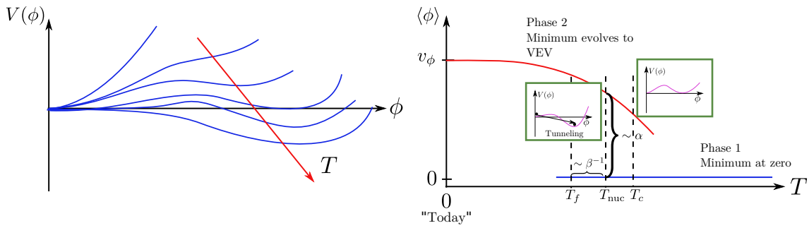
Figure 1: Left: Qualitative temperature dependence of a typical potential in particle physics developing a barrier and new global minimum as temperature drops. Right: Schematic illustration of the temperature dependence of the VEV (order parameter) in a FPT. Shown are also the two important temperatures T_c and T_{\text{nuc}} at which the minima are degenerated and at which the nucleation probability reaches one bubble per Hubble volume, respectively. The temperature at which the transition is completed is denoted by T_f .
