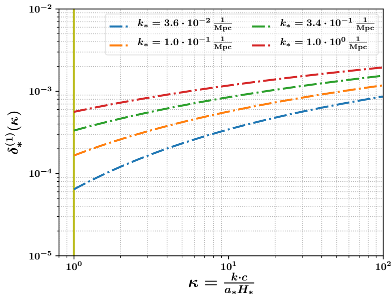
Figure 7: The estimated first order density fluctuations from the matter power spectrum in Eq. (103) as a function of dimensionless wave number for different times. Here k_* = \frac{a_* H_*}{c} . The \kappa -axis and the Hubble horizon shown in yellow are given in terms of the respective time for each of the curves.
