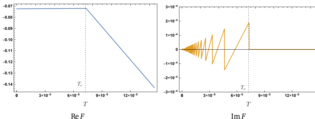
Figure 3: Real and imaginary parts of the free energy as a function of the temperature. We observe a distinctive saw-like pattern in the imaginary part which will also appear in SYK. The parameters used for these plots are k = 1, S_0 = 10^3, N(j) = 0, j_0 = 3 \times 10^{-3} .
