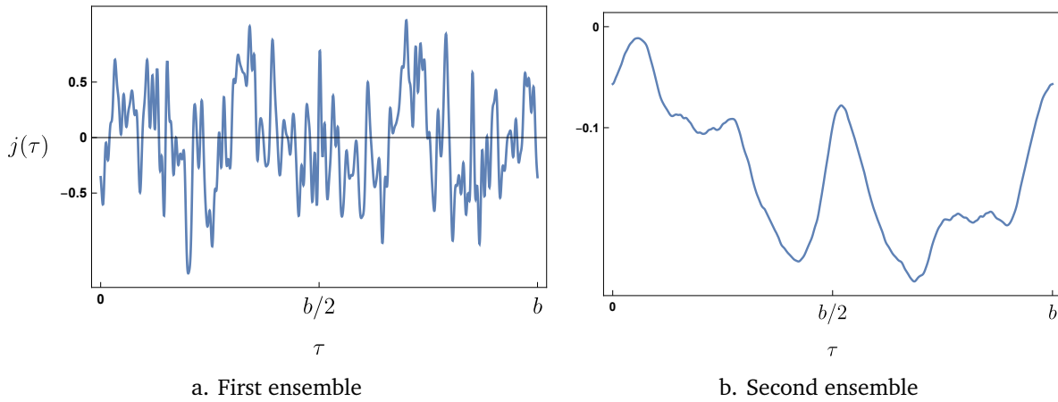
Figure 5: Typical realization of j(\tau) .
