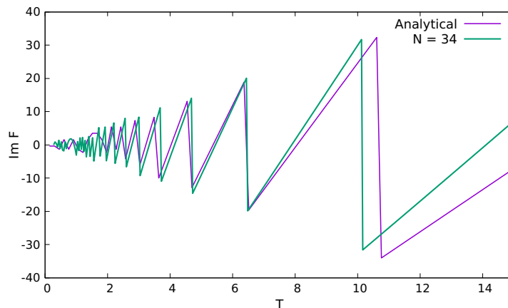
Figure 12: Imaginary part of the free energy for z = 9e^{i\pi/6} . We find an excellent agreement with the gravity prediction Eq. (51) with fitting parameters that provide an effective relation between the SYK and the gravity system parameters.
