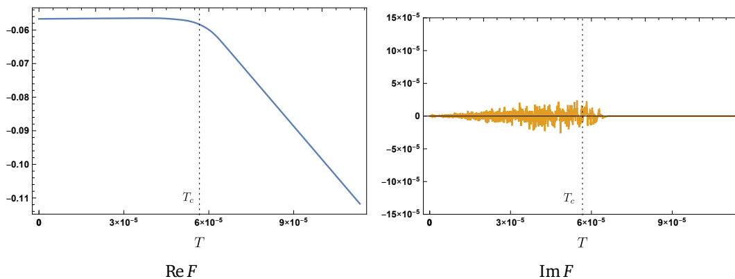
Figure 8: Quenched average over 100 realization of j(\tau) in the first ensemble (55). The parameters used for the plot are k = 1, S_0 = 10^3, J = 0.1 . The vertical scale for the imaginary part is adapted for one realization so that we see that it averages to zero. T_c is defined as the mean of the critical temperatures of the different realizations.
