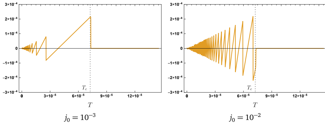
Figure 4: Imaginary part of the free energy as a function of the temperature. We see that j_0 is related to the number of oscillations. A similar behavior will be observed in SYK for the dual parameter r . The parameters used for these plots are k = 1, S_0 = 10^3, N(j) = 0 .
