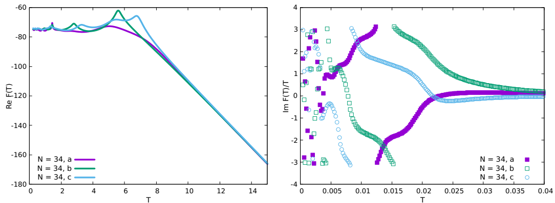
Figure 9: Left: Real part of the free energy for a single disorder realization of the Hamiltonian (92) for N = 34 and z = re^{i\theta} = 0 . We consider a few disorder realizations in order to illustrate the dependence of the results on the choice of random couplings. This dependence is relatively minor. In all cases, we do observe clearly a flat part for low temperature and a rather abrupt decreases at a finite temperature T_c consistent with a first order phase transition. This is similar to both the prediction of gravity of the previous section and also the free energy after ensemble average of the two-site complex SYK [48] related to a Euclidean wormhole. Right: Imaginary part of the free energy for the same parameters. Results are rather sensitive to the details of the disorder realization.
