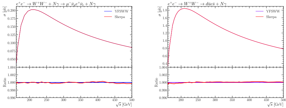
Figure 4: Total cross-section for hadronic and leptonic decay channel of e^+e^- \rightarrow W^+W^- .
