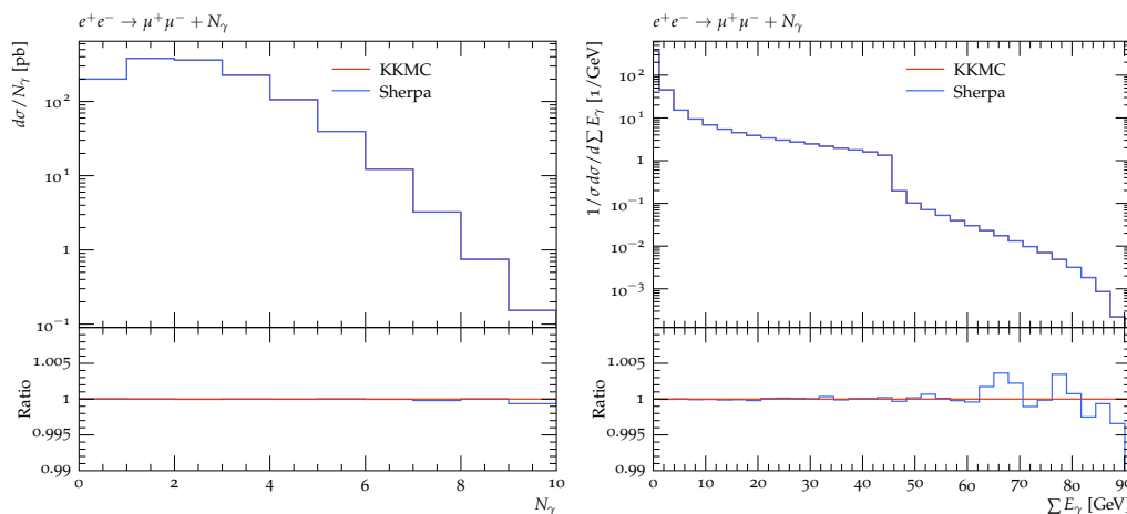
Figure 3: The total number of photons for both ISR and FSR (left), and the total sumeend photon energy (right), comparing SHERPA with KKMC.
