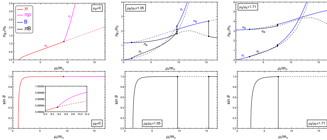
Figure 6: Same as Fig. 5, but as functions of the isospin chemical potential for three different values of the baryon chemical potential.
