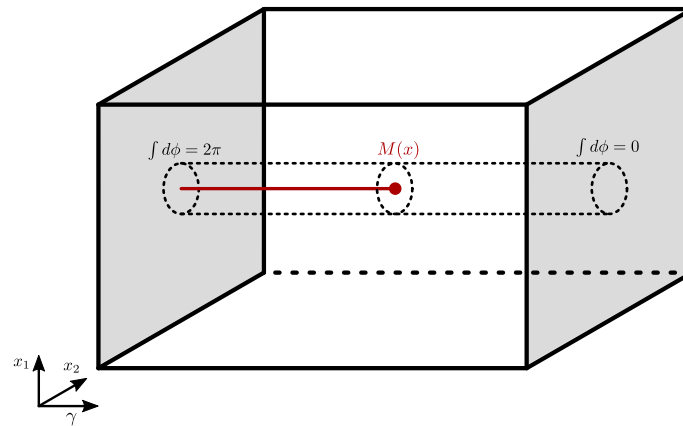
Figure 2: Smooth deformation of the field configuration in the presence of dynamical monodromy defects in a 2d compact scalar theory. The monodromy defect (line in red) ends on the monodromy defect operator M(x) . As a result, configurations with different monodromy charge are smoothly connected.
