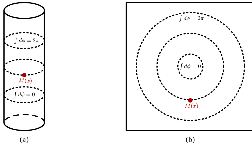
Figure 1: Compact scalar cylinder quantization with a monodromy operator. a) represents the theory on the cylinder. The quantization is along the circle and, as x is crossed, the state monodromy jumps. b) depicts the radial quantization and is related to a) by a conformal transformation.
