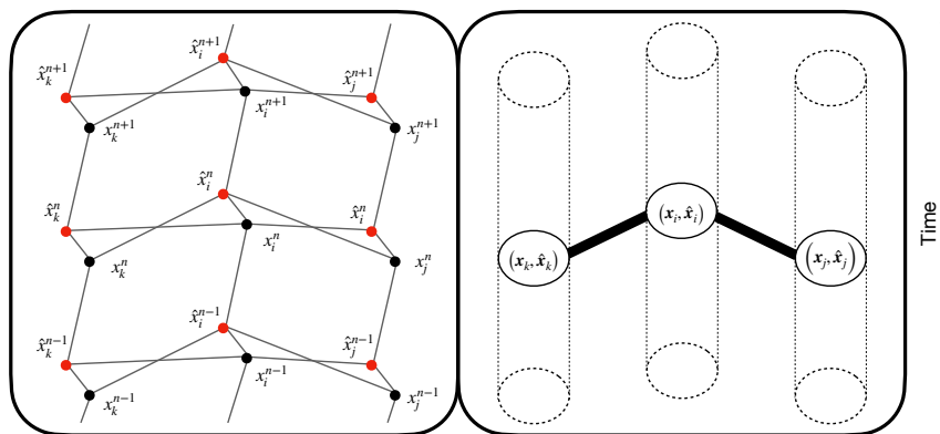
Figure 1: Graphical model associated with the dynamical partition function. Left panel: graphical model associated with the dynamical partition function of Eq. (5), where each node corresponds to a variable and each edge corresponds to a factor in the associated factor graph. The time direction is indicated by the arrow on the far right. The factor graph of the model exhibits numerous short loops, rendering a direct cavity approach infeasible. Right panel: graphical model associated with the dynamical partition function when grouping together, for each node i , the trajectories \mathbf{x}_i and \hat{\mathbf{x}}_i . The factor graph maintains the same structure as the underlying interaction graph.
