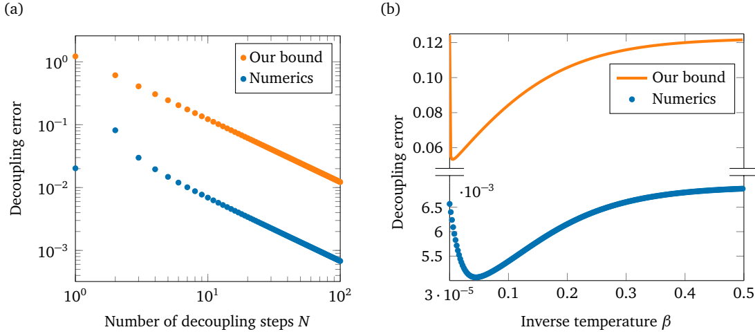
Figure 1: Carr-Purcell dynamical decoupling error for a qubit coupled to monochromatic boson field via a dephasing interaction. The Hamiltonian is given in Eq. (2), and the dynamical decoupling is performed by repetitive \pi -rotations (Pauli \sigma_x pulses). The initial state is |+\rangle \langle +| \otimes \rho_B , where \rho_B is the Gibbs state of the bosonic bath with inverse temperature \beta . We fix the total evolution time to t = 1 and choose \omega_S = 1 , \omega_B = 10 and f = 0.1 . The orange curve shows our analytical bound (C.72) and the blue curve shows a numerical simulation, where we truncated the bosonic field in Fock space at dimension d = 10 . (a) Error as a function of the number N of decoupling cycles for fixed \beta = 1 . We see that the decoupling error decays as 1/N . Our bound captures the asymptotic behaviour of the decoupling error. (b) Error as a function of the inverse temperature \beta for fixed N = 10 . We see that the decoupling error first decays with increasing \beta and then increases as \mathcal{O}(\sqrt{\beta}) . Finally, the error saturates at a constant due to finite N . The error decay for small \beta is lightly visible in our bound (which scales as \mathcal{O}(1/\sqrt{\beta}) in this regime), and it correctly captures the \mathcal{O}(\sqrt{\beta}) scaling and eventual saturation for larger \beta .
