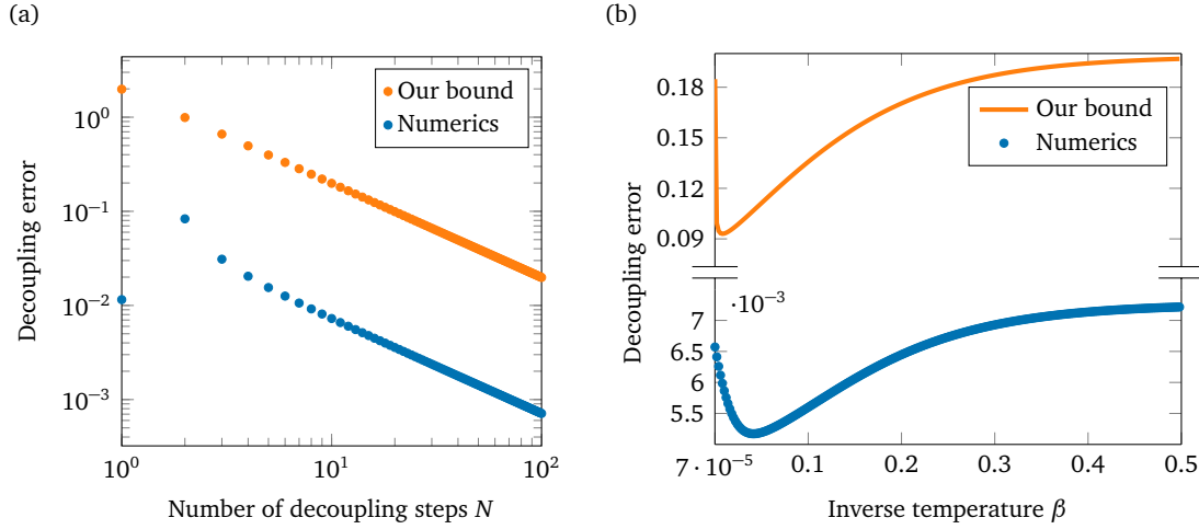
Figure 3: Dynamical decoupling error for a qubit coupled to monochromatic boson field via a quantum Rabi interaction. The Hamiltonian is given in Eq. (67) and dynamical decoupling is performed by repetitive pulse cycles through the Pauli group \mathcal{V} = \{I, \sigma_x, \sigma_y, \sigma_z\} . The initial state is |0\rangle\langle 0| \otimes \rho_B , where \rho_B is the Gibbs state of the bosonic bath with inverse temperature \beta . We fix the total evolution time to t = 1 and choose \omega_S = 1 , \omega_B = 10 and f = 0.1 . The orange dots show our analytical bound (C.77) and the blue dots show a numerical simulation, where we truncated the bosonic field in Fock space at dimension d = 10 . (a) Error as a function of the number n of decoupling cycles for fixed \beta = 1 . We see that the decoupling error decays as 1/N . Our bound captures this asymptotic behaviour of the decoupling error. (b) Error as a function of the inverse temperature \beta for fixed N = 10 . We see that the decoupling error first decays with increasing \beta and then increases as \mathcal{O}(\sqrt{\beta}) . Finally, the error saturates at a constant due to finite N . The error decay for small \beta is lightly visible in our bound (which scales as \mathcal{O}(1/\sqrt{\beta}) in this regime), and it correctly captures the \mathcal{O}(\sqrt{\beta}) scaling and eventual saturation for larger \beta .
