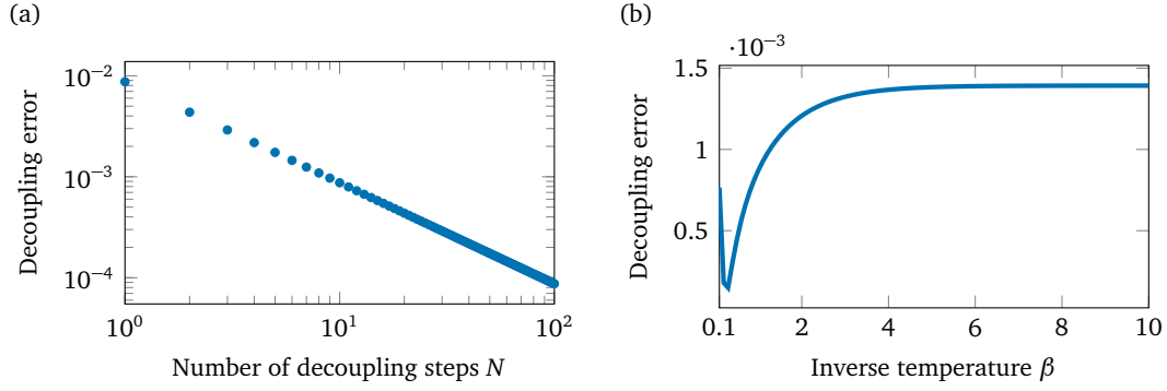
Figure 4: Dynamical decoupling error for a qubit coupled to an infinite number of bosonic modes via a Jaynes–Cummings interaction. The Hamiltonian is given in Eq. (70) for B = \sigma_- , (\omega_k)_{k \in \mathbb{N}} = (k)_{k \in \mathbb{N}} and (f_k)_{k \in \mathbb{N}} = \left(\frac{f}{k^2}\right)_{k \in \mathbb{N}} with f = 0.1 . Dynamical decoupling is performed by repetitive pulse cycles through the Pauli group \mathcal{V} = \{I, \sigma_x, \sigma_y, \sigma_z\} . The initial state is |0\rangle\langle 0| \otimes \rho_B , where \rho_B is the Gibbs state of the bosonic bath with inverse temperature \beta . We fix the total evolution time to t = 1 and choose \omega_s = 1 . The blue dots show our analytical bound for the decoupling error. (a) Error as a function of the number of decoupling cycles N for fixed \beta = 1 (This bound is obtained by inserting Eqs. (C.82)–(C.84) into Eq. (C.44)). We see that the decoupling error decays as 1/N . (b) Error as a function of \beta for fixed N = 10 (This bound is obtained by inserting Eqs. (C.82)–(C.84) into Eq. (C.44)). We see that the decoupling error increases as \mathcal{O}(\sqrt{\beta}) for small \beta and eventually saturates at a constant due to finite N .
