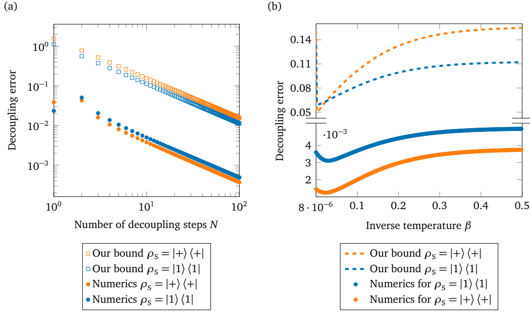
Figure 2: Dynamical decoupling error for a qubit coupled to monochromatic boson field via a flip-flop (Jaynes–Cummings) interaction. The Hamiltonian is given in Eq. (63) and dynamical decoupling is performed by repetitive pulse cycles through the Pauli group \mathcal{V} = \{I, \sigma_x, \sigma_y, \sigma_z\} . The initial state is \rho_S \otimes \rho_B , where \rho_B is the Gibbs state of the bosonic bath with inverse temperature \beta and \rho_S is either |+\rangle\langle+| (orange) or |1\rangle\langle 1| (blue). We fix the total evolution time to t = 1 and choose \omega_S = 1 , \omega_B = 10 and f = 0.1 . (a) Error as a function of the number N of decoupling cycles for fixed \beta = 1 . The empty squares show our analytical bound (Eq. (C.74) for \rho_S = |0\rangle\langle 0| and Eq. (C.75) for \rho_S = |+\rangle\langle+| ) and the filled dots show a numerical simulation, where we truncated the bosonic field in Fock space at dimension d = 10 . We see that the decoupling error decays as 1/N . Our bound captures this asymptotic behaviour of the decoupling error. (b) Error as a function of the inverse temperature \beta for fixed N = 10 . The dashed lines are our bound (Eq. (C.74) for \rho_S = |0\rangle\langle 0| and Eq. (C.75) for \rho_S = |+\rangle\langle+| ) and the dots are a numerical simulation, where we truncated the bosonic field in Fock space at dimension d = 10 . We see that the decoupling error first decays with increasing \beta and then increases as \mathcal{O}(\sqrt{\beta}) . Finally, the error saturates at a constant due to finite N . The error decay for small \beta is lightly visible in our bound (which scales as \mathcal{O}(1/\sqrt{\beta}) in this regime), and it correctly captures the \mathcal{O}(\sqrt{\beta}) scaling and eventual saturation for larger \beta .
