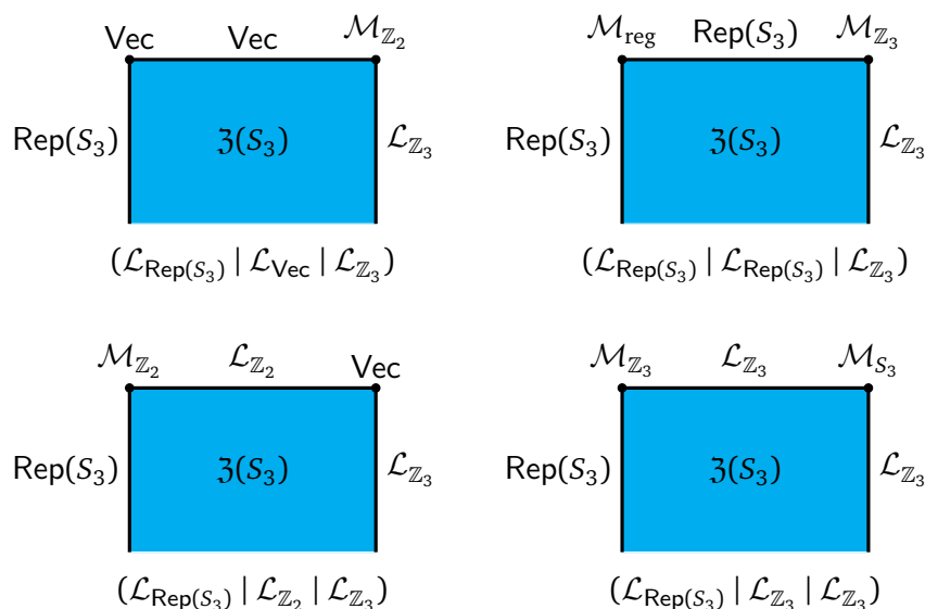
Figure 12: Four Boundary SymTFTs describing a (1+1)d \text{Rep}(S_3)/\mathbb{Z}_2 SSB phase with \text{Rep}(S_3) symmetry.
