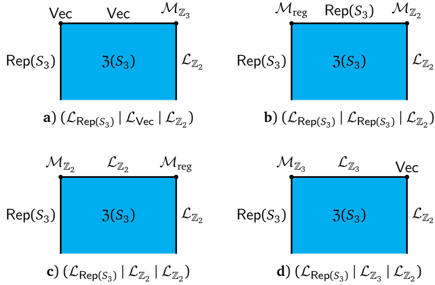
Figure 11: Four Boundary SymTFTs for the \mathbb{Z}_2 SSB phase of \text{Rep}(S_3) , with boundary.
