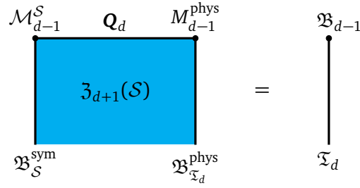
Figure 2: Simplified depiction of the Boundary SymTFT used throughout the paper. Note that the interface between the (d-1) -charge \mathbf{Q}_d and \mathfrak{B}^{\text{sym}} is a (d-1) -module category. The same applies to the interface between \mathbf{Q}_d and \mathfrak{B}^{\text{phys}} in case the theory is a gapped phase.
