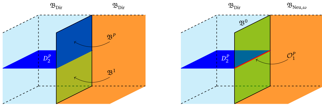
Figure 5: Minimal doublet of BCs (left) and singlet BC (right) for \mathbb{Z}_2 0-form symmetry in (2+1)d.
