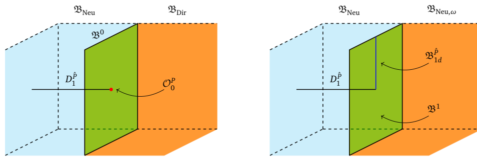
Figure 6: Minimal singlet BC \mathfrak{B}^0 (left) and doublet of BCs \mathfrak{B}^1, \mathfrak{B}^{\hat{P}} (right) for \mathbb{Z}_2 1-form symmetry in (2+1)d. Note that \mathfrak{B}_{1d}^{\hat{P}} is the BC \mathfrak{B}^{\hat{P}} compactified to a line.
