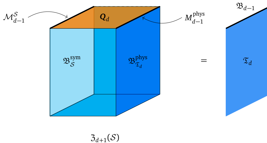
Figure 1: 3d depiction of the Boundary SymTFT: The bulk SymTFT is given in terms of the (d + 1) -dimensional TQFT \mathfrak{Z}_{d+1}(S) and the two boundary conditions: the gapped symmetry boundary \mathfrak{B}_S^{\text{sym}} and (not necessarily gapped) physical boundary \mathfrak{B}_{\mathfrak{T}_d}^{\text{phys}} . The boundary SymTFT extends this to another gapped boundary condition – indicated here by \mathbf{Q}_d , which has interfaces \mathcal{M}_{d-1}^S and M_{d-1}^{\text{phys}} with the other two boundary conditions. The interval compactification shown on the right hand side, results in a theory \mathfrak{T}_d with boundary \mathfrak{B}_{d-1} . From the perspective of generalized charges of the symmetry S , the SymTFT description of boundary conditions is in terms of the ends of \mathbf{Q}_d , i.e. so-called (d - 1) -charges.
