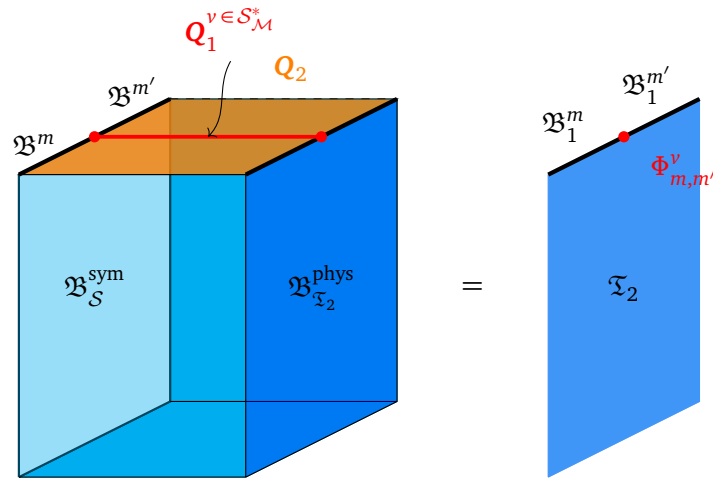
Figure 3: Boundary changing operators in (1+1)d. The interface between \mathfrak{B}^{\text{sym}} and \mathfrak{Q}_2 (shown in orange) is the module category \mathcal{M} , with m, m' \in \mathcal{M} . The boundary changing operator is 0-charge Q_1^v , where v \in \mathcal{S}^*_{\mathcal{M}} , which stretches between \mathcal{M} and M^{\text{phys}} . The interaction points become the boundary changing operator \Phi after interval compactification.
