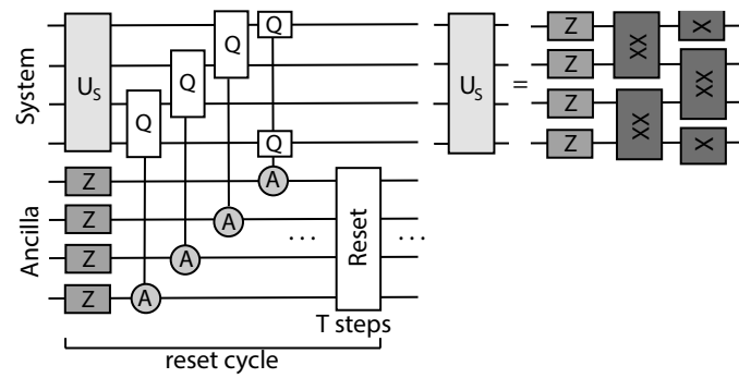
Figure 3: Scheme of our dissipative transverse field Ising realization, similar to Refs. [3, 9] and realistic to implement with a digital quantum computer. In this setup, the system’s qubits are coupled to ancillary ones. After every T system-ancilla-coupling propagations, ancilla qubits are reset to the spin-down state.
