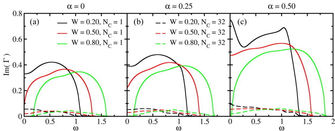
Figure 7: The imaginary part of hybridization function integrated over momentum \text{Im}(\Gamma(\omega)) for different disorder strength: W = 0.20 (weak disorder), 0.50 (intermediate disorder), and 0.80 (strong disorder), and different SOC strength: \alpha = 0 (absence of SOC, panel (a)), 0.25 (panel (b)), and 0.50 (panel (c)), for N_c = 1 and 32 .
