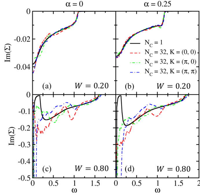
Figure 2: Imaginary part of the self-energy, \text{Im} \underline{\Sigma}(\mathbf{K}, \omega) , computed using DCA for disordered two-dimensional systems without Rashba SOC (left panels) and with SOC at \alpha = 0.25 (right panels). Panels (a) and (b) show results for weak disorder ( W = 0.20 ) at N_c = 1 (CPA) and N_c = 32 , evaluated at high-symmetry momenta \mathbf{K} = (0, 0) , (\pi, 0) , and (\pi, \pi) . Panels (c) and (d) show the corresponding results at stronger disorder ( W = 0.80 ).
