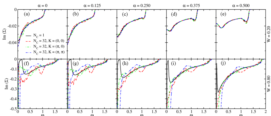
Figure 6: The imaginary part of self-energy \text{Im}\Sigma(\mathbf{K}, \omega) for different values of \alpha : \alpha = 0 (no SOC, (a), (f)), \alpha = 0.125 ((b), (g)), \alpha = 0.25 ((c), (h)), \alpha = 0.375 ((d), (i)), and \alpha = 0.50 ((e), (j)). The top panels ((a)-(e)) show the self-energy at W = 0.20 (weak disorder), and the bottom panels ((f)-(j)) show the self-energy at W = 0.80 (stronger disorder). We note that panels (a), (c), (f), and (h) restores panels (a), (b), (c), and (d) of Figure 2 in the main text, respectively.
