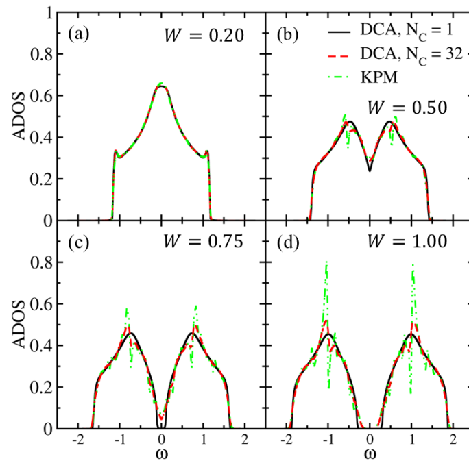
Figure 4: Benchmarking of ADOS computed using DCA for cluster sizes N_c = 1 and N_c = 32 against results obtained from the KPM for disordered two-dimensional systems with Rashba SOC ( \alpha = 0.25 ) at various disorder strengths. KPM calculations were performed on a 300 \times 300 square lattice with periodic boundary conditions using 1024 Chebyshev moments and 10^3 disorder realizations for statistical averaging.
