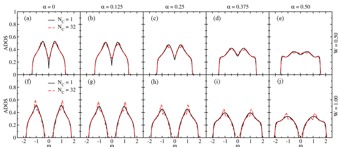
Figure 5: The average density of states (ADOS) calculated using DCA for different values of \alpha : \alpha = 0 (no SOC, (a), (f)), \alpha = 0.125 ((b), (g)), \alpha = 0.25 ((c), (h)), \alpha = 0.375 ((d), (i)), and \alpha = 0.50 ((e), (j)), and two disorder strength: W = 0.50 (intermediate disorder strength, in (a)-(e)), and W = 1.00 (large disorder strength, in (f)-(j)). We note that panels (a), (c), (f), and (h) restores panels (c), (d), (e), and (f) of Figure 1 in the main text, respectively.
