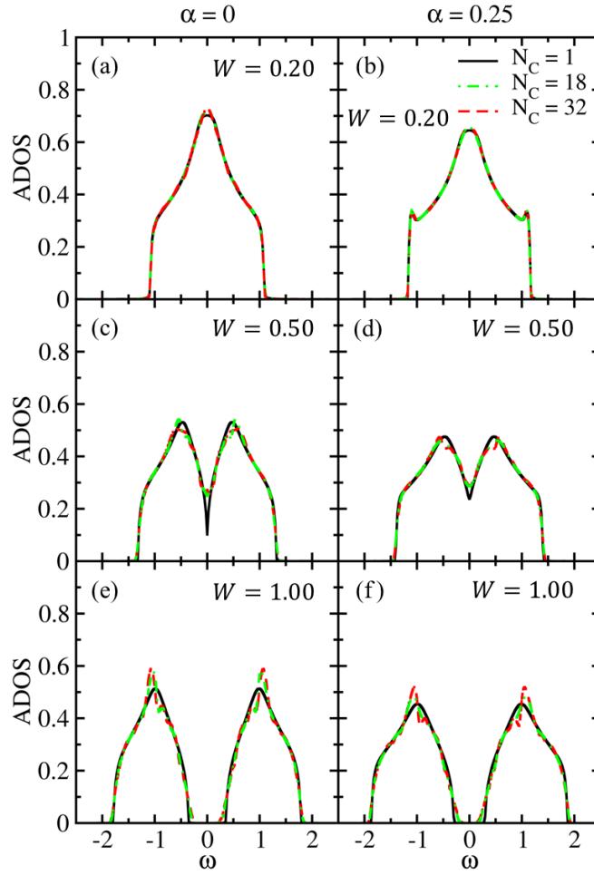
Figure 1: ADOS computed using DCA for disordered two-dimensional electronic systems without Rashba SOC (left panels) and with SOC at \alpha = 0.25 (right panels). Panels (a)-(f) compare results for N_c = 1 (CPA, black solid curves), N_c = 18 (green dot-dashed curves) and N_c = 32 (red dashed curves) at increasing disorder strengths: W = 0.20 ((a), (b)), W = 0.50 ((c), (d)), and W = 1.00 ((e), (f)).
