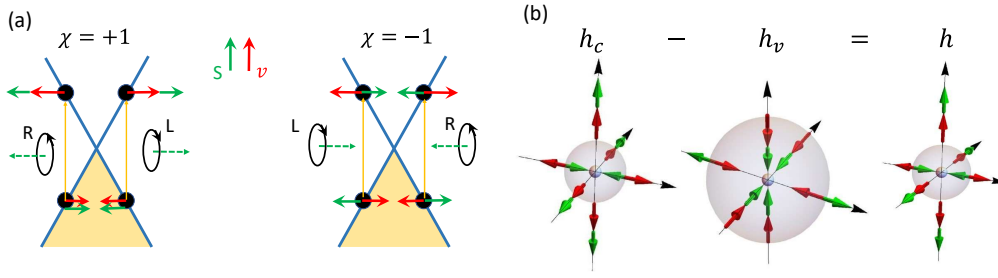
Figure 1: Schematic diagram of the circular optical spin injection for a pair of Weyl nodes connected by inversion symmetry (a) and momentum-space spin texture (b). In (a), the coupling to the circular polarization of light is determined by the Berry curvature in the conduction band, which is parallel (for \chi = +1 ) and antiparallel (for \chi = -1 ) to the velocity v . The dashed green arrow in (a) shows the angular momentum of light, which is transferred to the Weyl Fermions, accounting for the difference between the green arrows in the conduction and valence band. When the chirality is flipped from +1 to -1, the projection of spin on v is also flipped, suggesting a locked helicity and chirality, which collaborate constructively to yield a nontrivial induced magnetization from chiral light. For (b), the three plots show the spin texture for helicity in the conduction ( h_c ) and valence band ( h_v ), and their difference ( h ).
