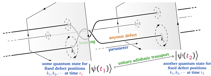
Figure 22: The quantum adiabatic theorem asserts that the sufficient slow (adiabatic) braiding of worldlines of anyonic defects in a 2-dimensional quantum material acts on the gapped ground states by unitary braid representation operators.
