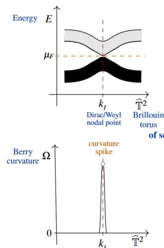
Figure 17: Band nodes in semimetals are submanifolds in the reciprocal space of crystal momenta where the gap between the valence band and the conduction band closes. These band nodes behave like source for Berry curvature.
