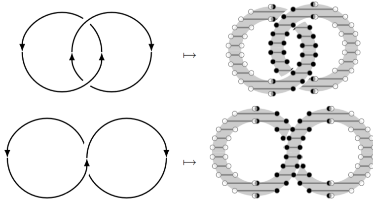
Figure 9: Loops in the configuration space of charged strings in the plane may be identified with (diagrams for) framed oriented links.
