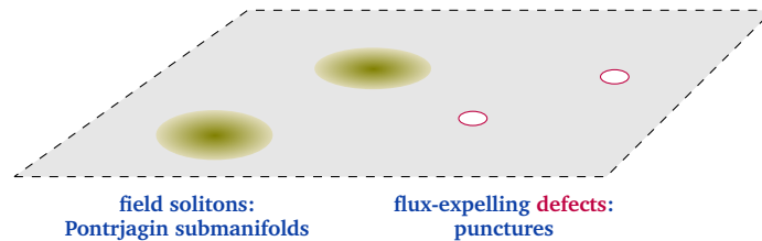
Figure 20: Due to the condition that charges vanish at infinity, punctures in the surface are the mathematical reflection of defects in the material where the magnetic flux is expelled.
