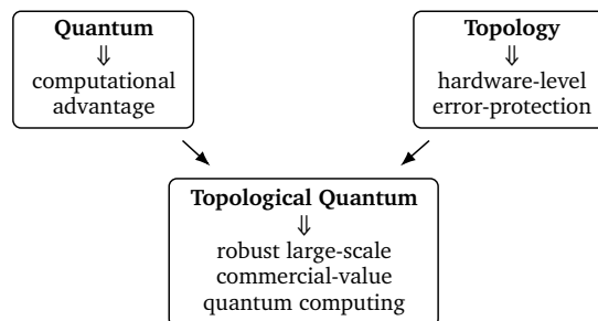
Figure 1: Topological quantum. In order to practically harness the computational power of quantum processes, quantum states need to be stabilized against decohering environmental noise. Apart from using quantum error correction at the software level, a plausibly necessary way to do so is by using topological quantum processes preventing quantum errors right at the hardware level.
