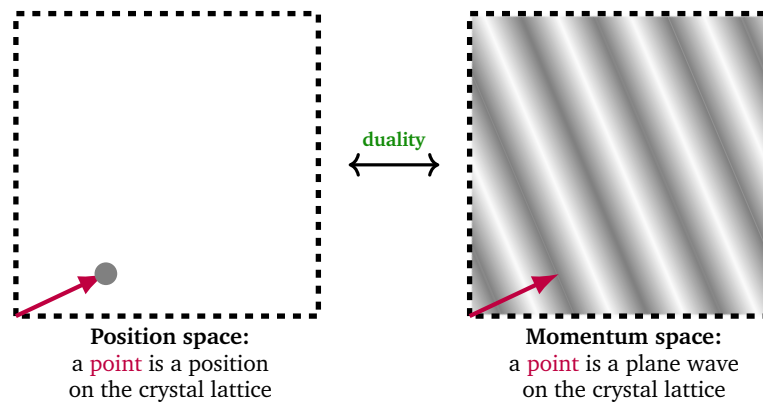
Figure 16: Crystal Fourier transform establishes a duality between the actual space inhabited by a crystalline sample, the "position space" and its "reciprocal space" of crystal momenta.
