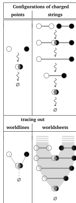
Figure 8: The continuous relations in configuration spaces of charged points and strings exhibit the pair annihilation/creation of oppositely charged (end-)points.
