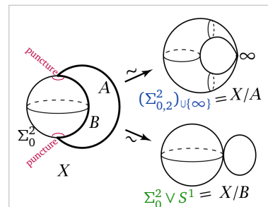
Figure 21: Topology change due to defects! (cf. [66, p 11]) Different to but not unlike the genon -proposal [8].
