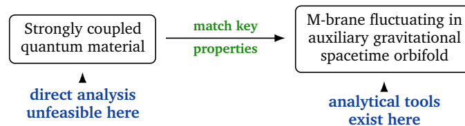
Figure 3: Geometric engineering of quantum systems on M-branes provides tools for analyzing otherwise elusive strongly coupled/correlated quantum phenomena.
