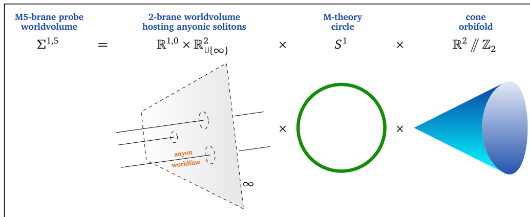
Figure 4: Brane diagram for geometric engineering of anyons on single M5-branes wrapping an orbi-singularity [137]. It is a subtle mechanism of flux-quantization [132] of the self-dual tensor-field on the M5 [54] that stabilizes [134] its anyonic soliton configurations.
