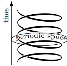
Figure 12: Worldline of a particle travelling around a compact dimension. In the limit of high momentum/boost the particle travels on a compactified light-cone.
