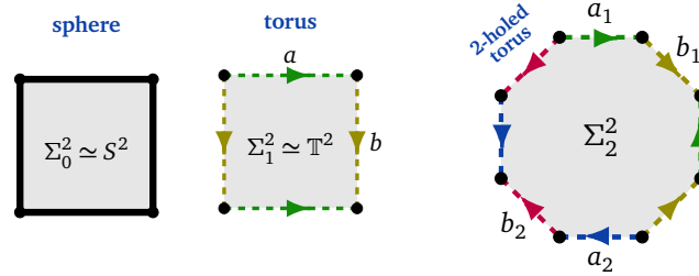
Figure 19: Fundamental polygons for closed surfaces.
