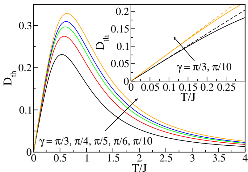
Figure 1: D_{\text{th}}(T) for different anisotropies. The inset compares the full result to the low-temperature asymptotics (dashed lines), see Eq. (3.8).
