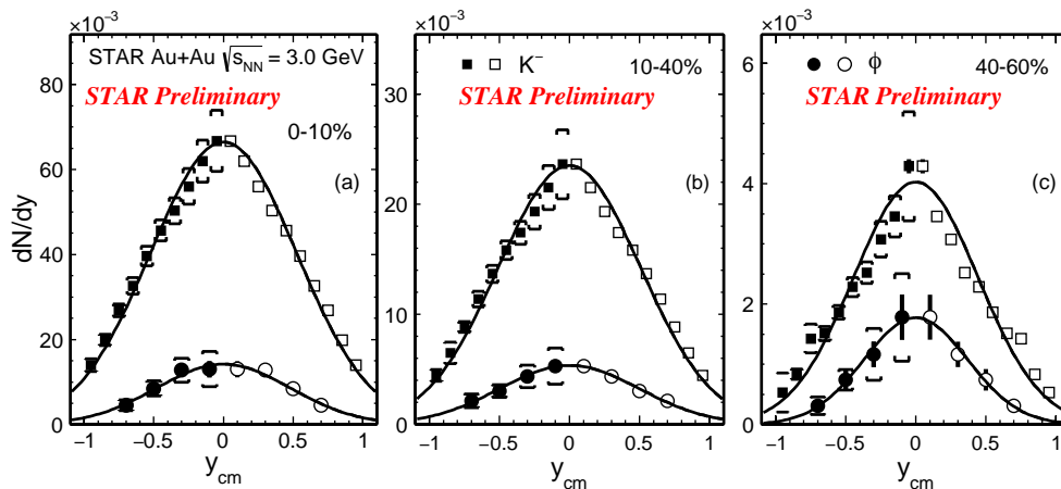
Figure 3: Rapidity distributions of K^- and \phi meson for various centrality regions, solid symbols are measured data, open ones are reflection. Yields obtained from integrating fit functions to the m_T spectra are fit with a Gaussian function.
