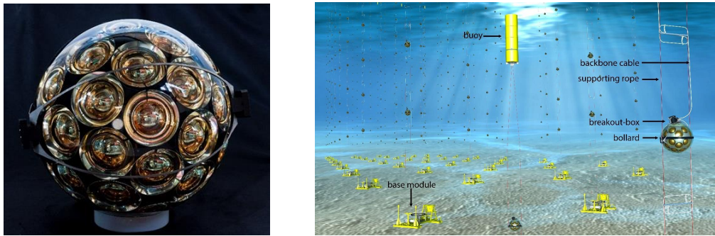
Figure 1: Left: View of a KM3NeT DOM. Right: Artistic view of the KM3NeT telescope. Detection Units equipped with DOMs and anchored at the sea bed are shown. Buoys at the top of each string keep the structure taut. At the level of each DOM a breakout of the backbone cable is visible. The Base Modules of DUs are connected to a Junction Box via cables deployed on the seafloor. The picture is not in scale.
