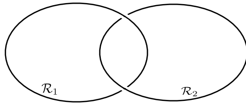
Figure 1: Hopf link.
