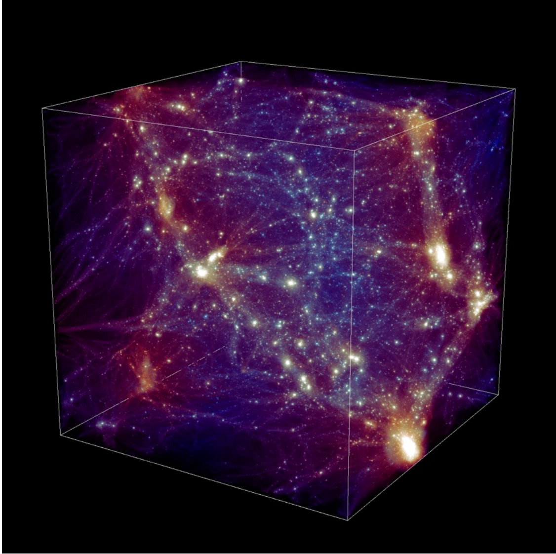
Figure 1: Color rendering of the dark matter particle distribution from a N-body simulation of a LCDM model. Dark matter halos are visible as clumps of different sizes. The color coding follows the mass of the halos, with large halos appearing redder and small halos appearing bluer. The characteristic filamentary structure of the Cosmic Web is striking. Simulation credit: RAMSES. Image credit: S. Colombi.
