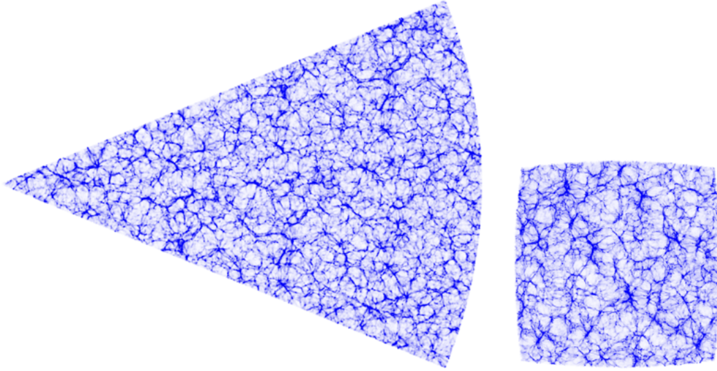
Figure 5: Left panel: Light cone as seen from an observer sitting at the tip of the triangle within a thin slice on the sky and up to redshift z = 0.5 . Right panel: Light cone as seen from the same observer but face-on for a thin slice in redshift around redshift z = 0.25 . Credit figure and simulation: T. Akieda-Codron.
