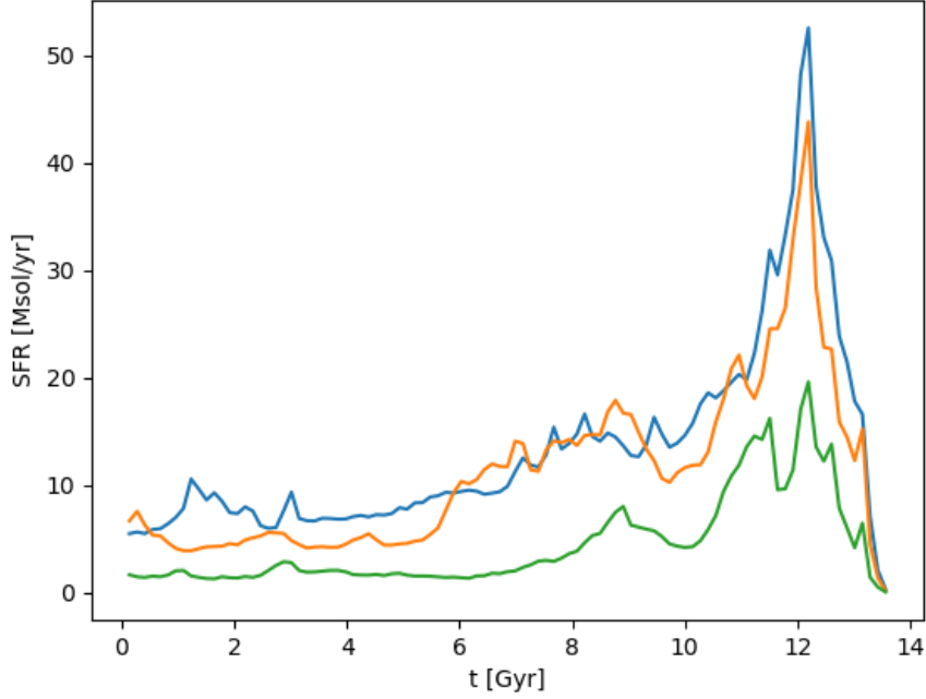
Figure 10: Star formation history for 3 different simulations of the same Milky-Way-like galaxy, based on the same dark matter halo simulated in the other Chapters, but varying the supernovae energy from E_{51} = 0 (blue line), to E_{51} = 2 (orange line) and finally to E_{51} = 4 (green line). Credit figure and simulation: R. Teyssier.
