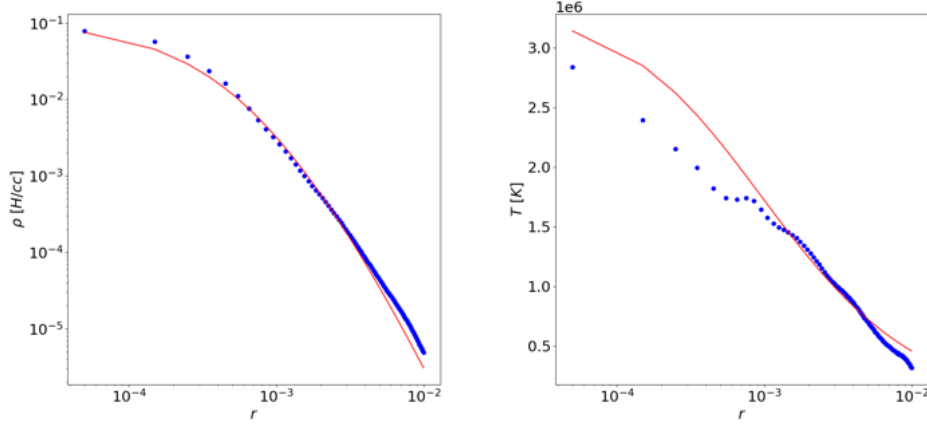
Figure 7: Left panel: gas density profile of the simulated halo in the non-radiative run. Blue dots represents the simulation data, while the red solid line show the analytical model. Right panel: Same but for the gas temperature. Credit figure and simulation: R. Teyssier.
