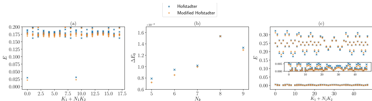
Figure 5. (a) The many-body spectrum at half filling for a 4-band ( \nu = 1=4 ) Hofstadter model and its modified version with the constant Berry curvature for a lattice of N_1 = N_2 = 9 = 8 sites. (b) The two-fold ground state degeneracy splitting \Delta E_0 at half filling for different systems of N_b bosons in a N_b = 2= lattice. When the lattice is perfectly square ( N_b = 8 ), the modified model has the same ground state energies as the original model hence the same ground state splitting. (c) The two-body spectrum for a system of N_1 = N_2 = 12 = 4 magnetic unit cells. The inset shows the lowest non-zero two-body energies per total momentum sector for both models.
