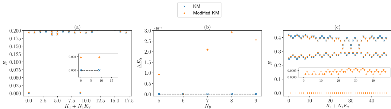
Figure 4. (a) The many-body spectrum at half filling for a 3-band ( \nu = 1=3 ) KM model and its modified version with the constant Berry curvature for a lattice of N_1 = N_2 = 9 = 8 sites. The inset shows the two-fold degenerate ground states. The dashed horizontal line is the zero energy line. (b) The two-fold ground state degeneracy splitting \Delta E_0 at half filling for different systems of N_b bosons in a N_b = 2= lattice. The dashed horizontal line is the zero ground state splitting line. When the lattice is perfectly square ( N_b = 6 ), the modified model has the same ground state energies as the original model hence the same ground state splitting. (c) The two-body spectrum for a system of N_1 = N_2 = 12 = 4 magnetic unit cells. The inset shows the lowest non-zero two-body energy per total momentum sector for the modified KM model.
